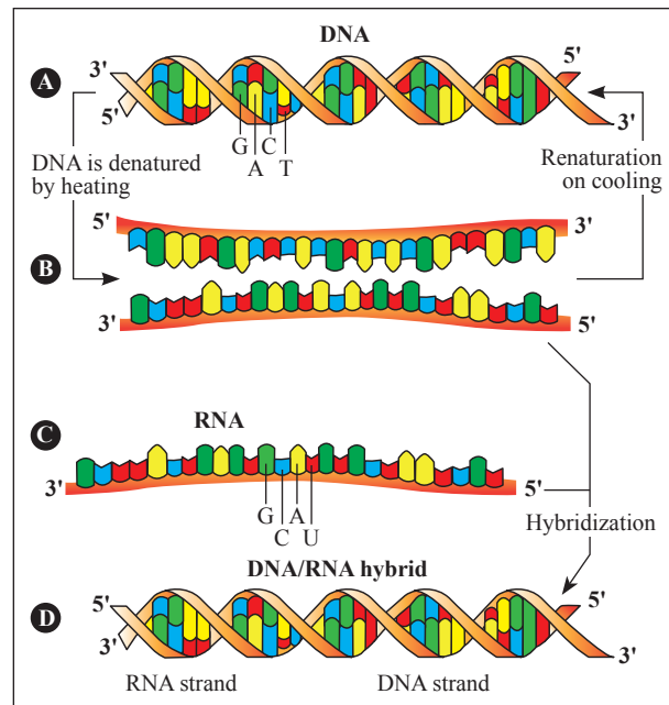
Figure 1. Nucleic Acid Hybridization
