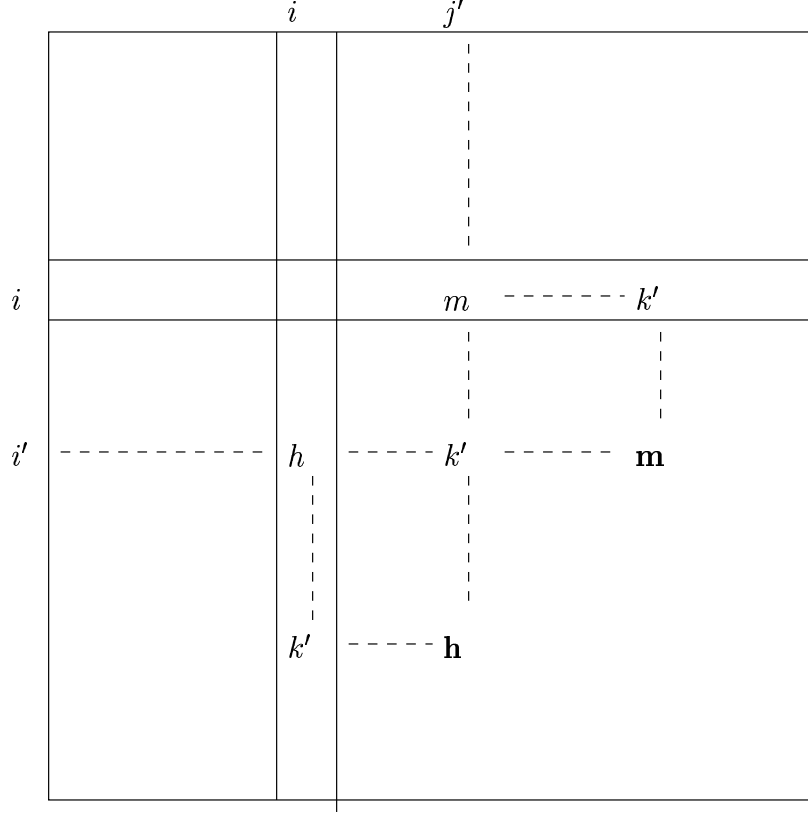
Figure 1: i' > i and j' > j
