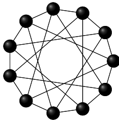
Figure 1: The \mathcal{A}_4 graph.
